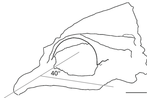
Fig. 8. Abactochromis labrosus , MRAC 99-041-P-1323, 114.0 mm SL; outline of neurocranium in lateral view. Superimposed gray lines show estimated angle of ethmovergerine block relative to parasphenoid. Scale bar 5 mm.
